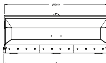
ICE-SCRAPING CUTTING EDGE Reinforced steel with ice-breaking geometry
